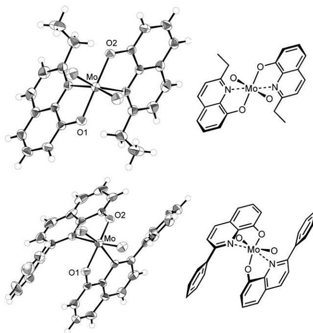
Figure 1. X-ray single-crystal structures of 9 (top) and 10 (bottom).
